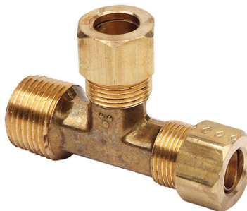
Brass Compression Run Tee
